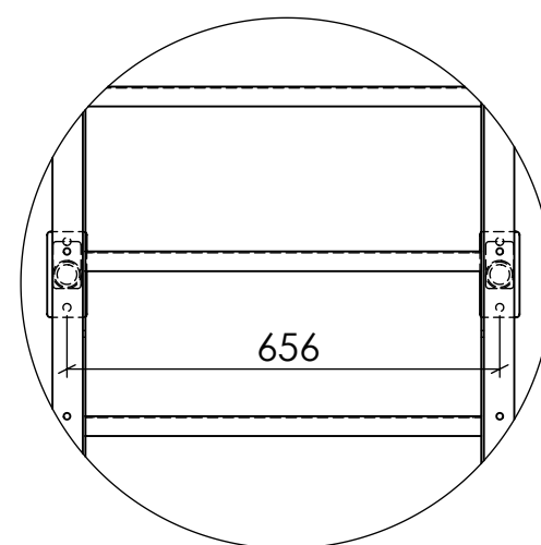
DETAIL G SCALE 2 : 25
